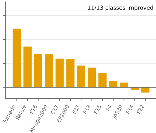
weak-uniform arm on weak classes
