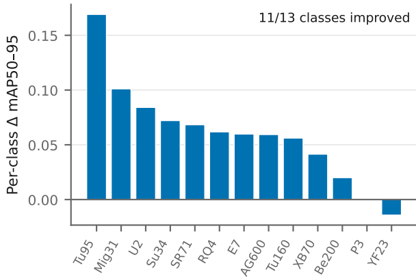
tail-uniform arm on tail classes
