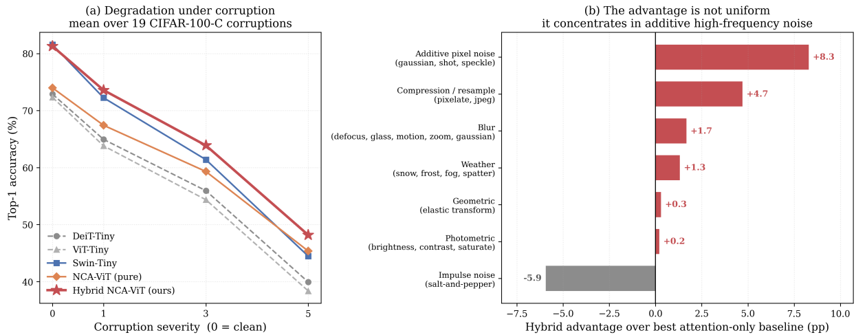
Fig. 2. Advantage over the best baseline, by corruption category — concentrated, not general.
