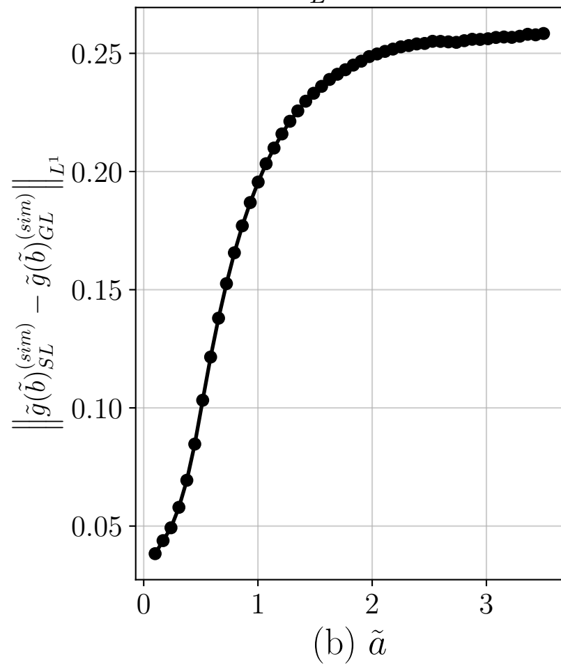
D_{L^1} vs. \tilde{a}
