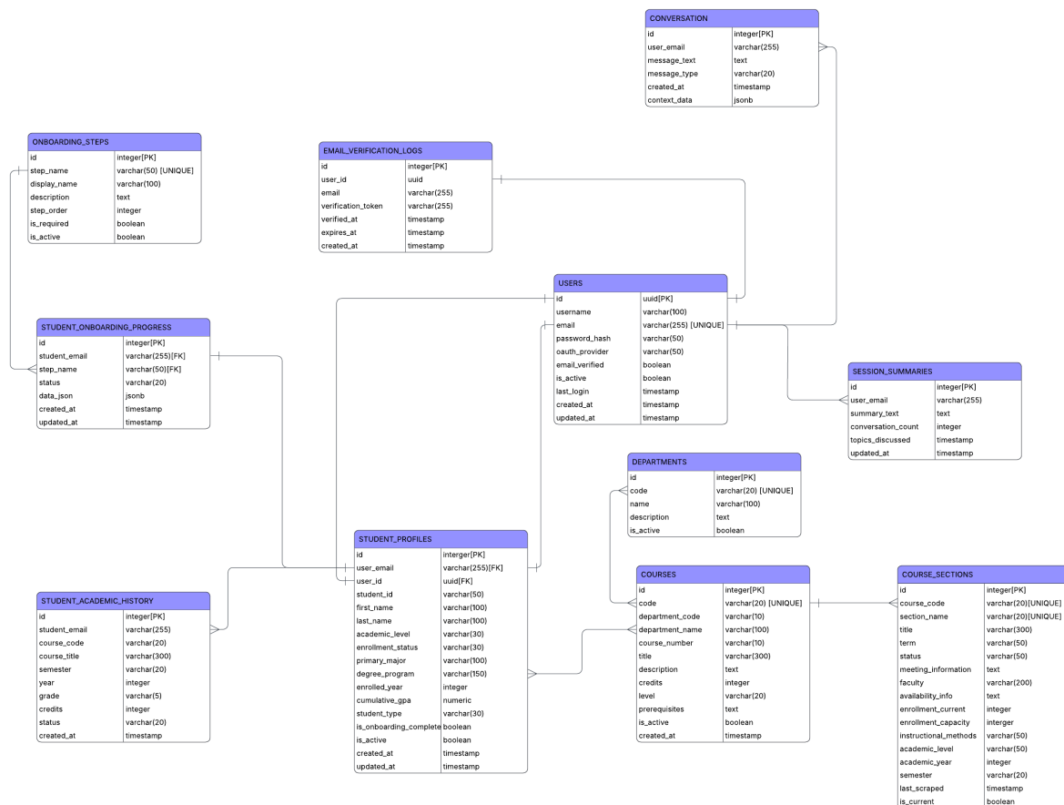
Figure 4.1: Entity Relationship Diagram (ERD) of the Academic Advising Chatbot System.
