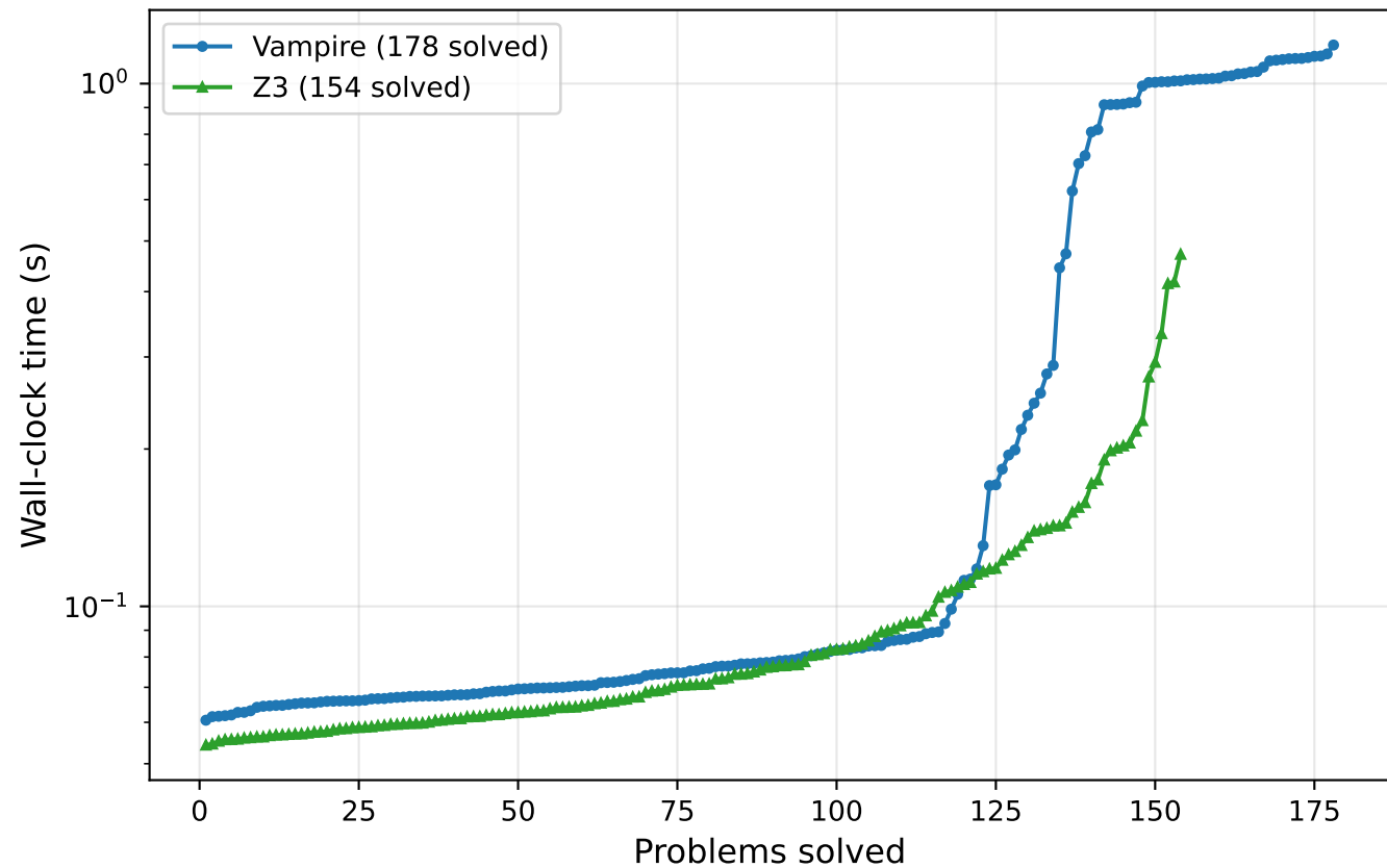
ODRL Benchmark Suite — Cactus Plot
