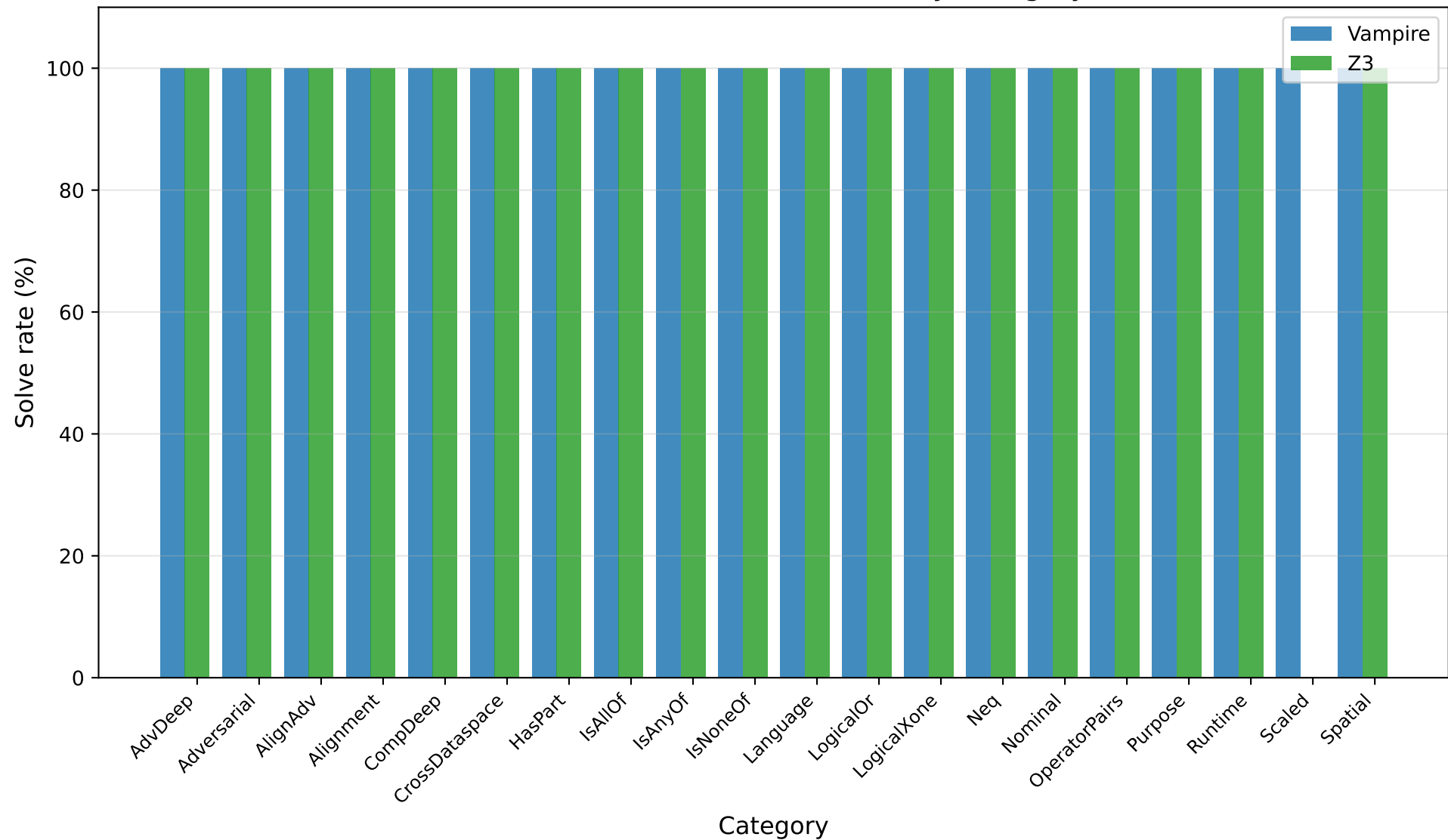
ODRL Benchmark — Solve Rate by Category
