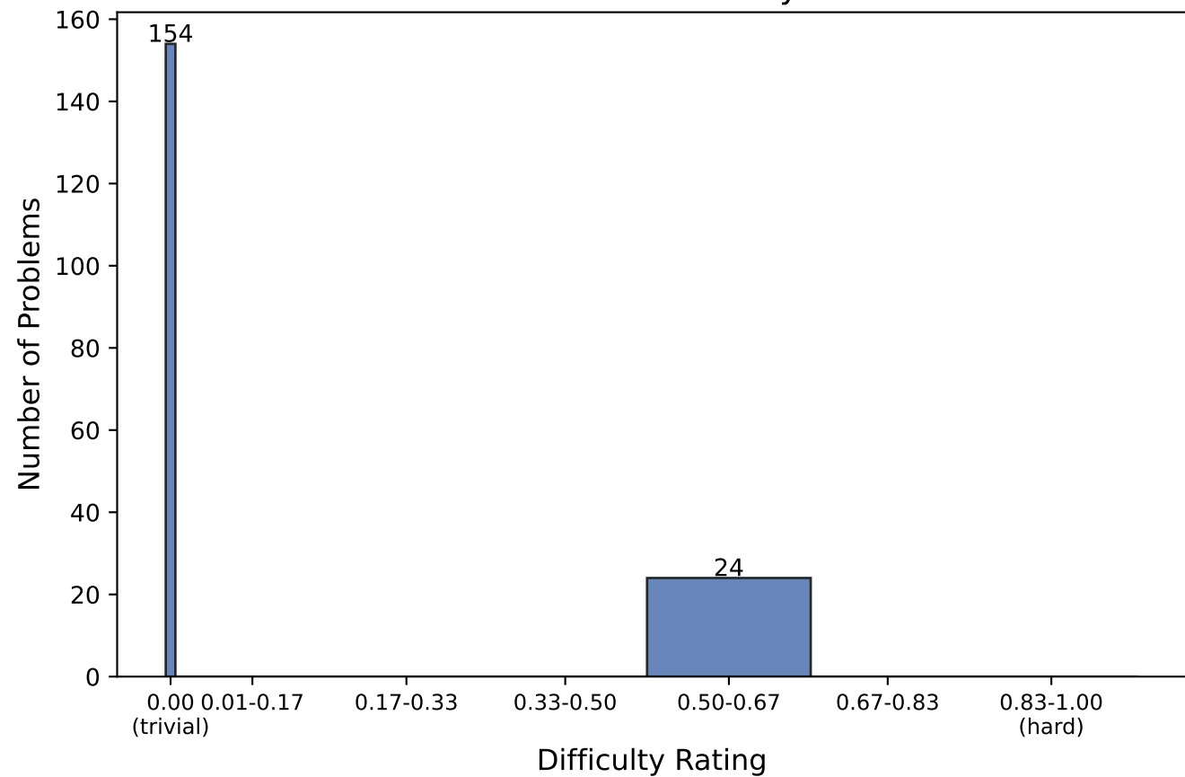
ODRL Benchmark — Difficulty Distribution
