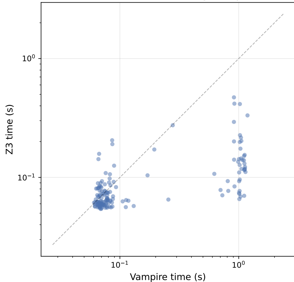
ODRL Benchmark — Timing Comparison
