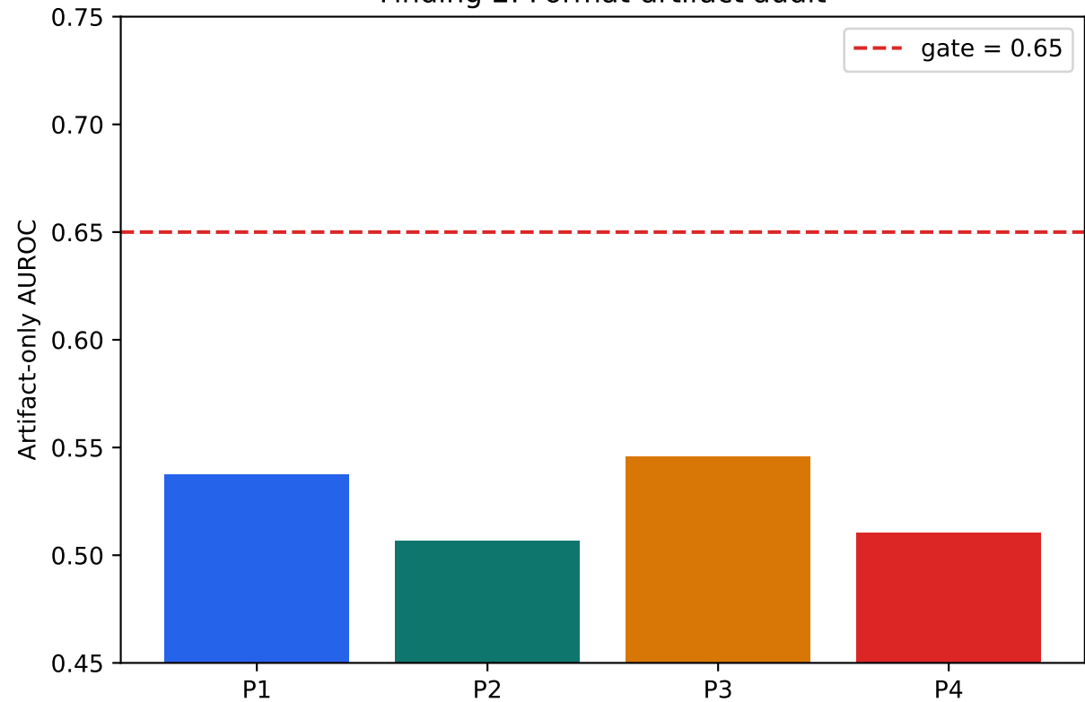
Finding 2: Format-artifact audit
