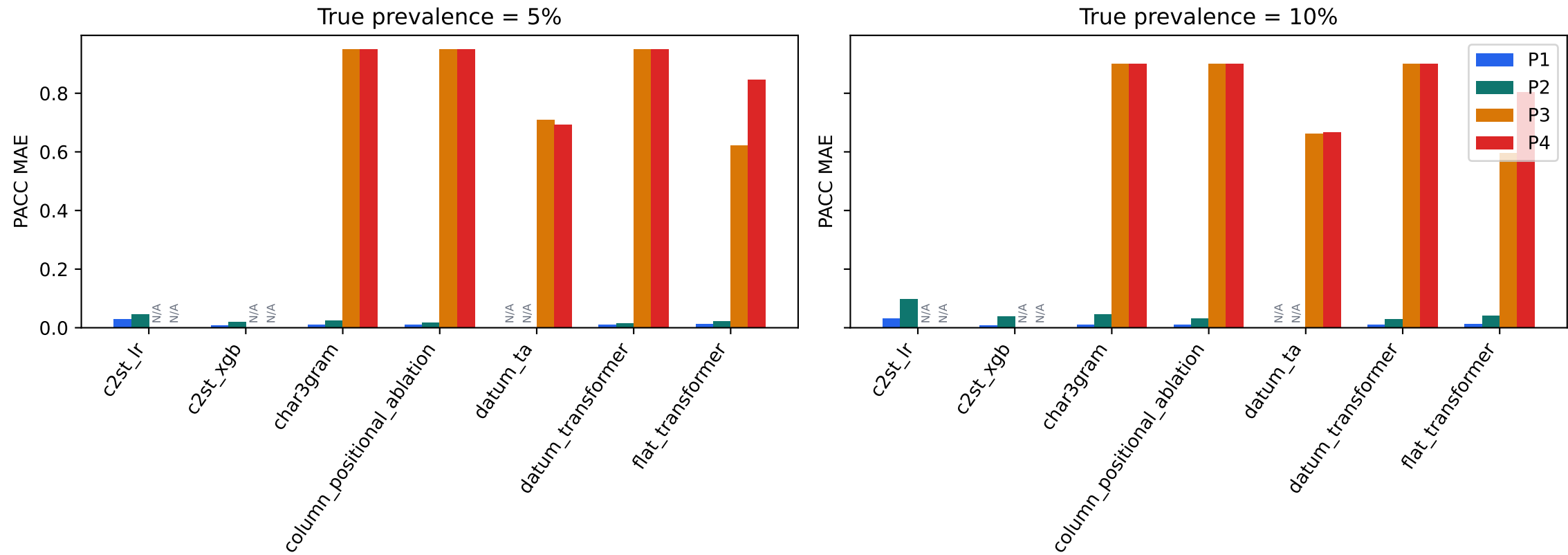
Finding 3: Low-prevalence estimation error (source-only, replace)
