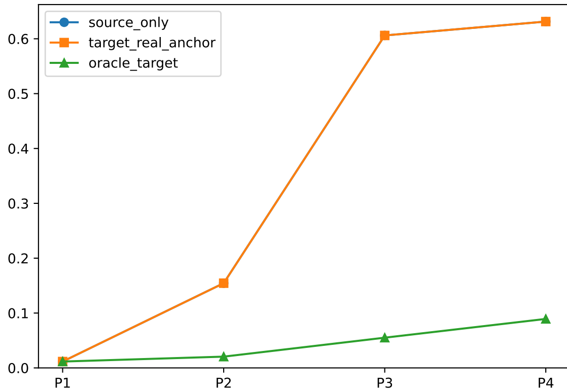
PACC prevalence MAE
