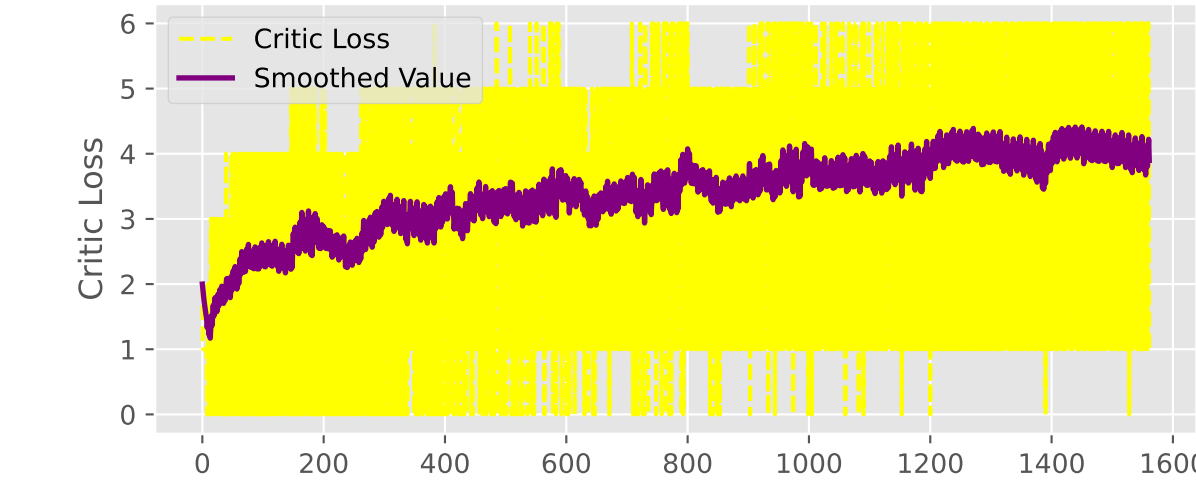
Critic Loss
