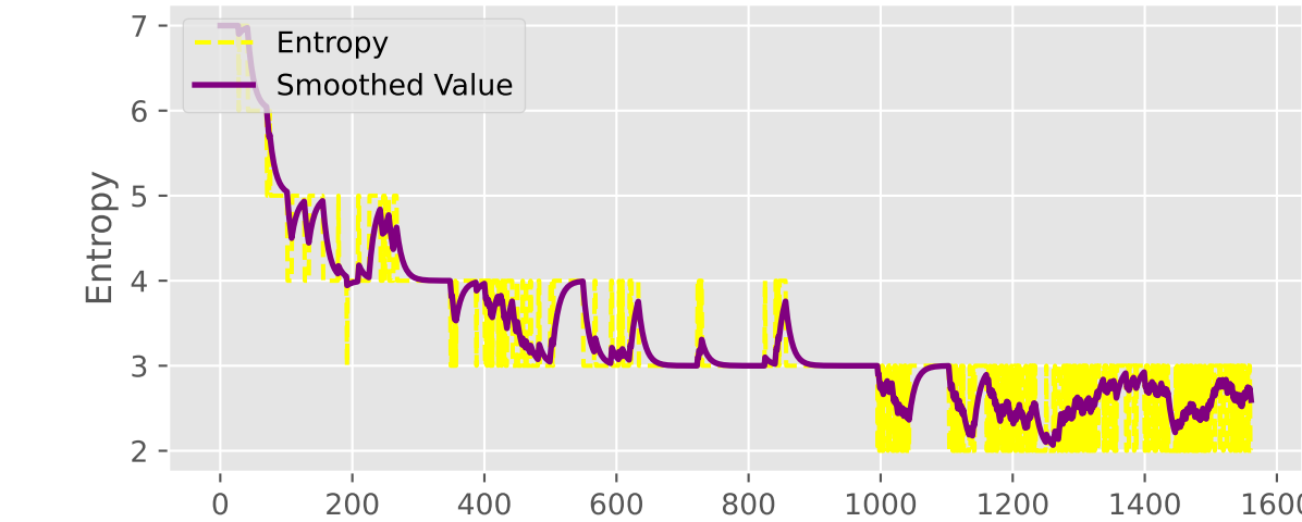
Entropy
