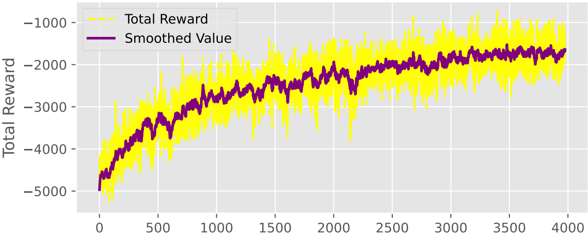
Total Reward
