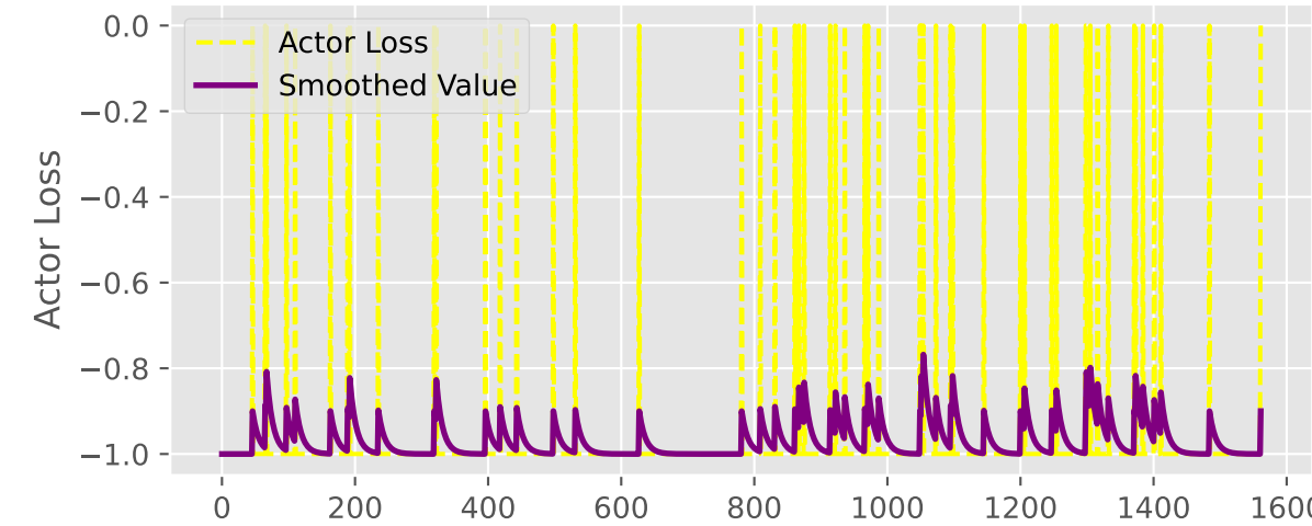
Actor Loss
