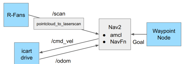
Fig. 7: Summary of the system during autonomous driving.
