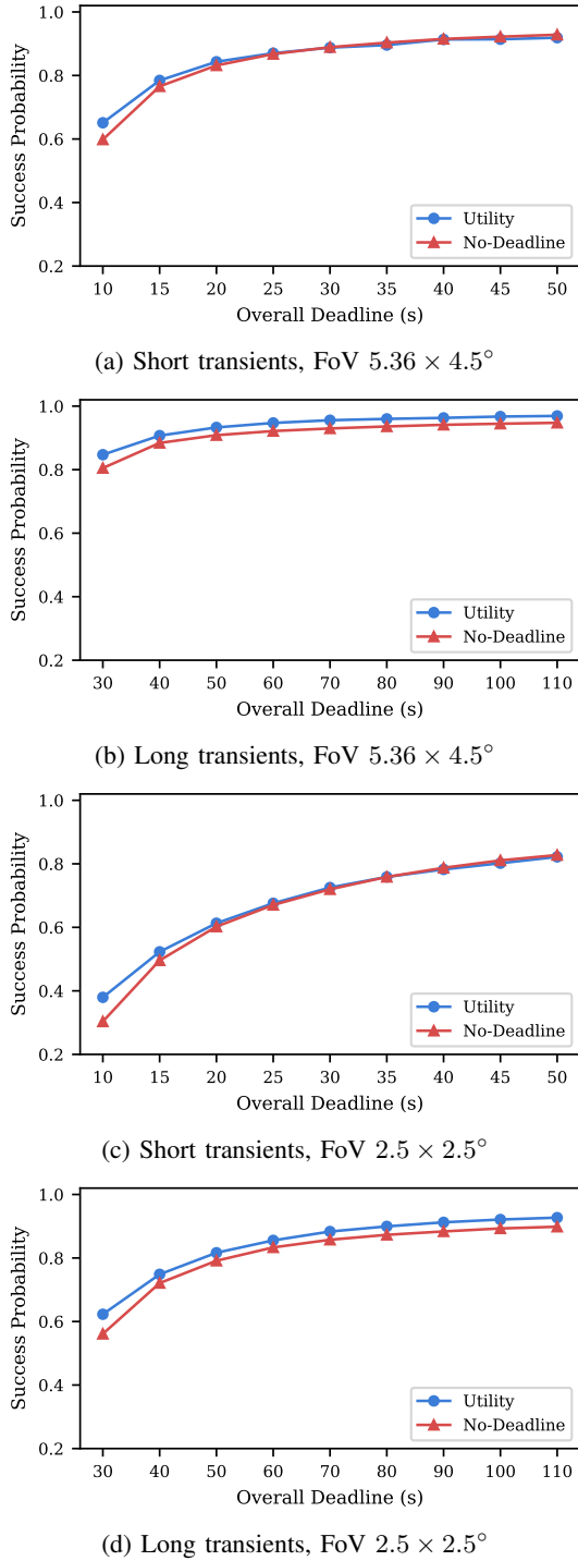
Fig. 11: Probability of successful transient detection by cooperating telescopes as a function of overall deadline D .
