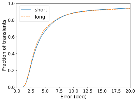
Fig. 7: Cumulative distribution of mapping errors for short and long transients. CDFs reach 1 at \sim 160^\circ error.
