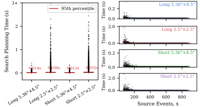
Fig. 6: Left : Box plots of search-planning time for short and long transients using different partner FoVs. Right : Search-planning time vs. number of source events. Most outliers have s < 200 .
