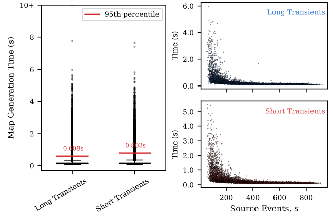
Fig. 5: Left : Box plots of map-generation times for 52,800 simulated TAPs on our target platform for both short and long transients. Right : Map-generation time vs. number of source events s = e - b . Most outliers occur when s < 350 .
