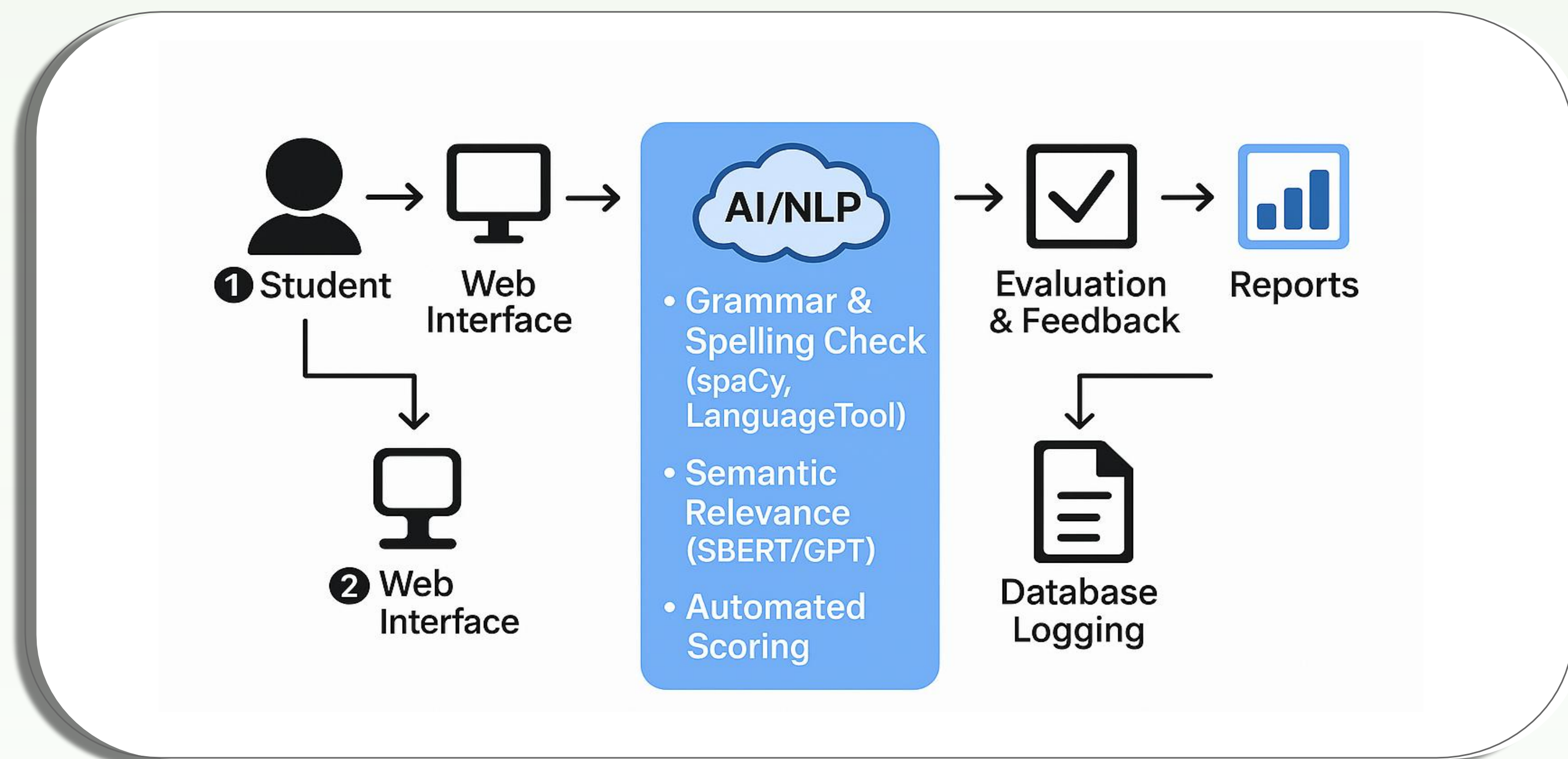
Fig. 1. CommuniqElevate Evaluation Flow
