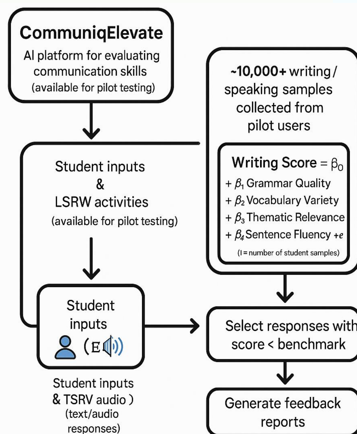
Fig. 3. AI Evaluation Workflow
