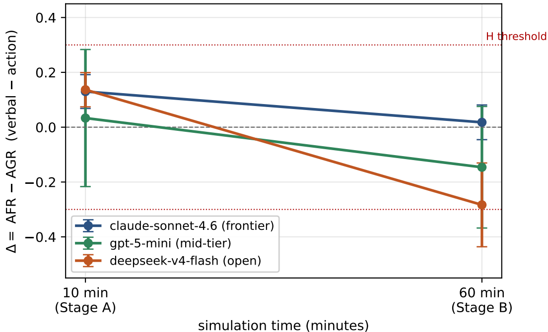
Verbal-action dissociation trajectory across model tiers
