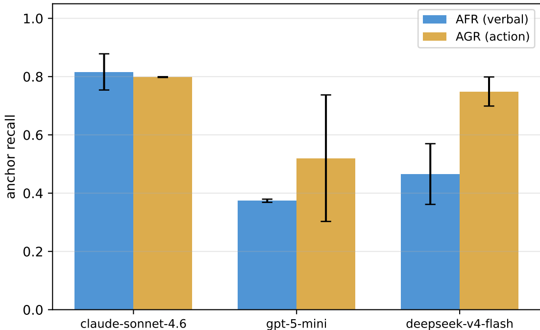
Dual probe at t = 1 sim-hour: anchor verbal vs action recall
