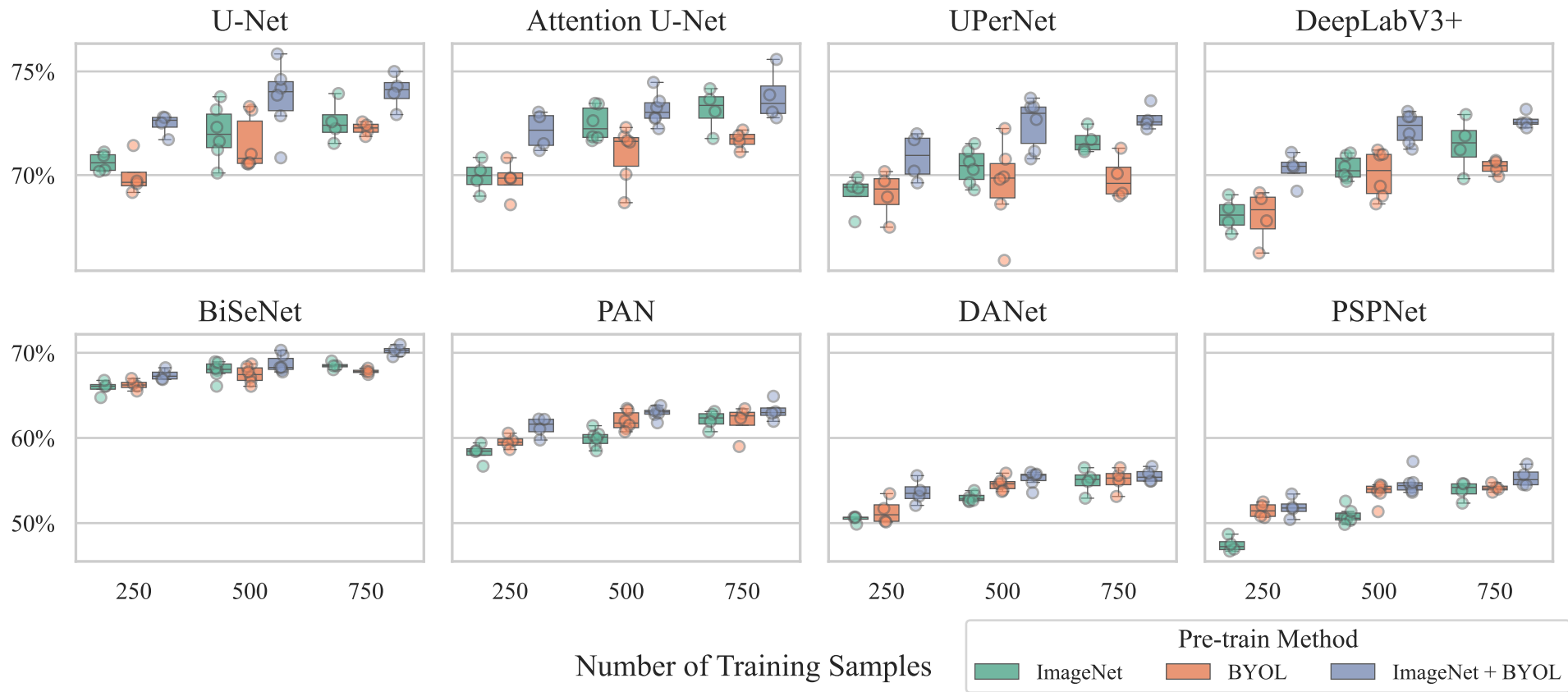
Macro F1-Score
