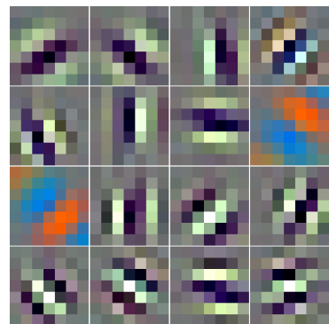
Convolutional Filters
