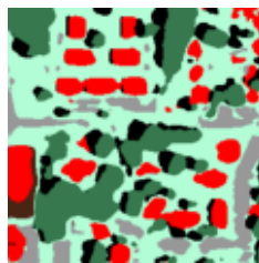
ImageNet Only
