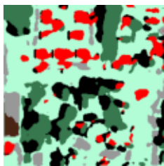
BYOL Only
