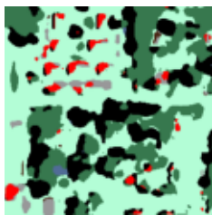
No Pre-training
