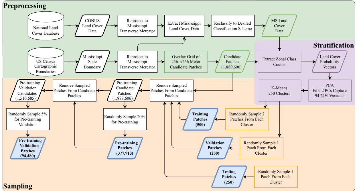
Figure 2: Flowchart of the stratified sampling process for selecting data for model training and validation GO BACK AND FIX ME!!!! .
