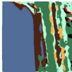
No Pre-training
