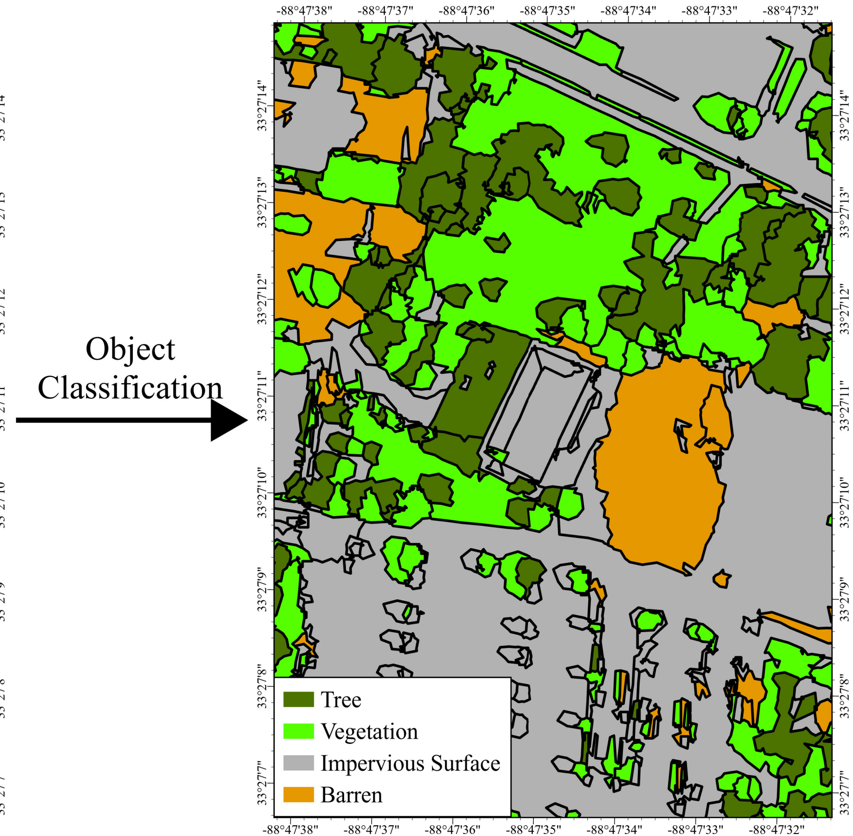
Classification Map
