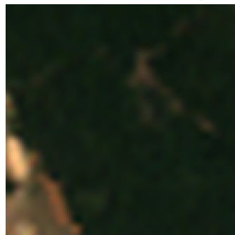
Sentinel-2 Input
