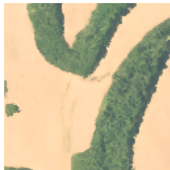
20 Steps
