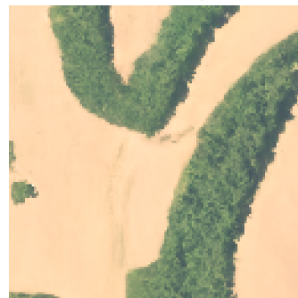
30 Steps
