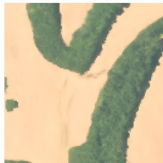
10 Steps
