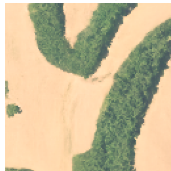
40 Steps
