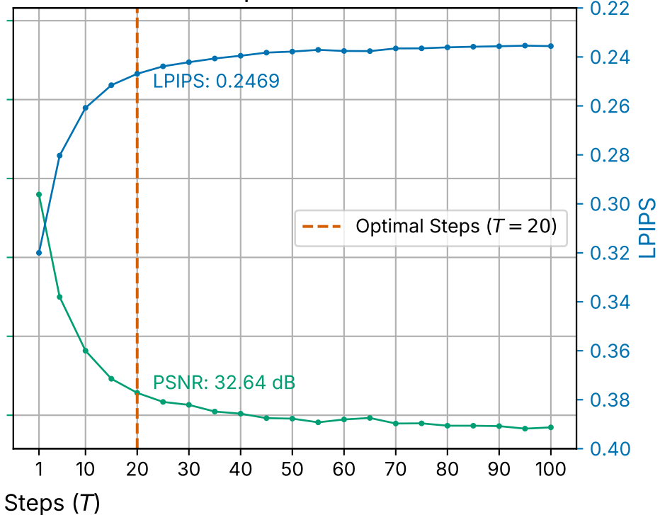
Midpoint Solver
