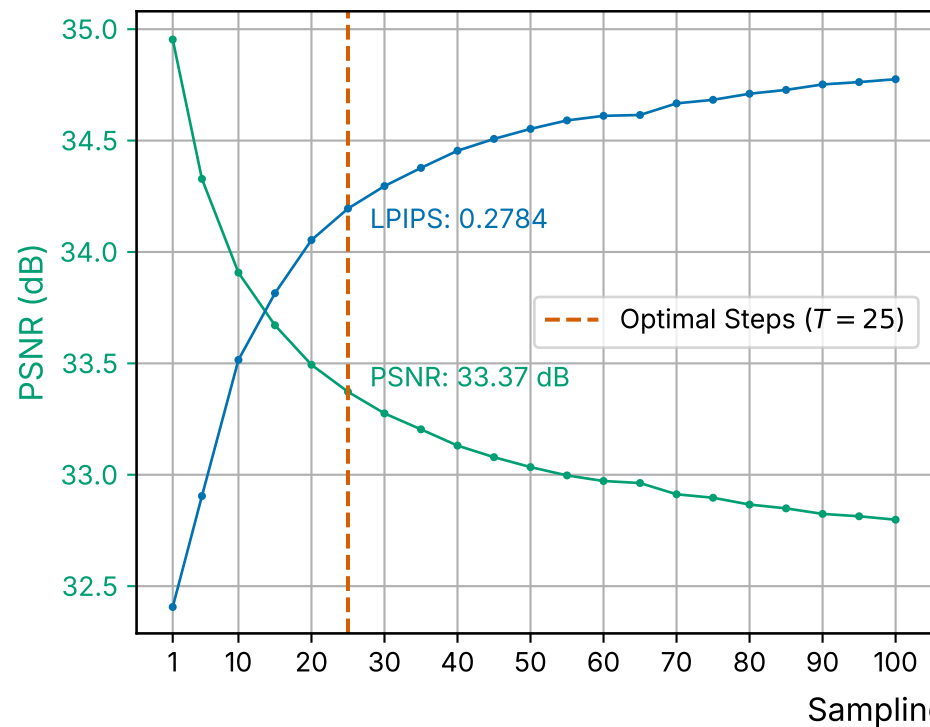
Euler Solver
