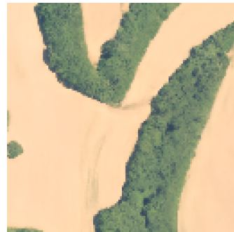
T = 25
