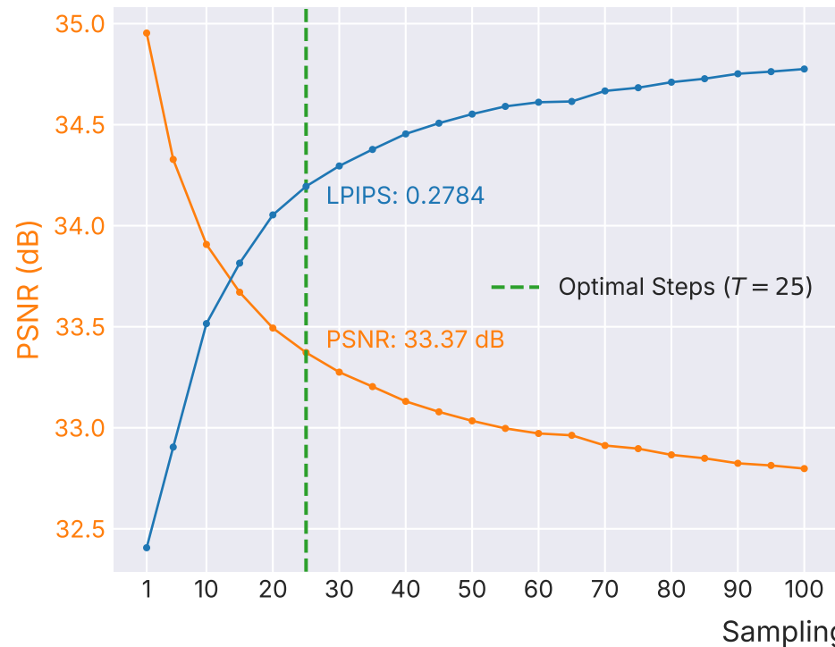
Euler Solver
