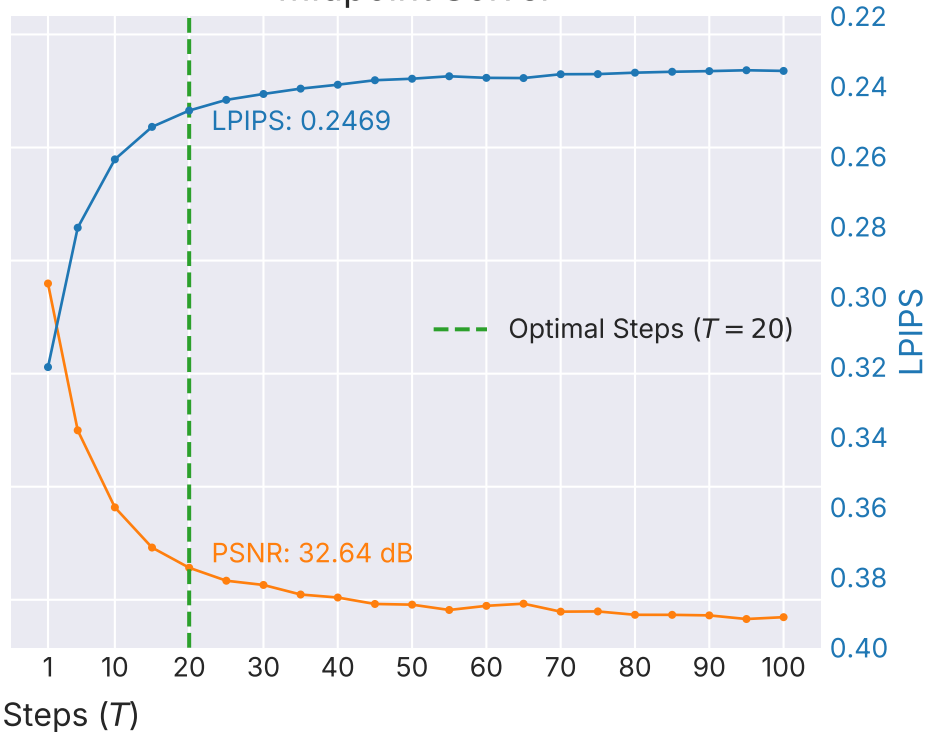
Midpoint Solver
