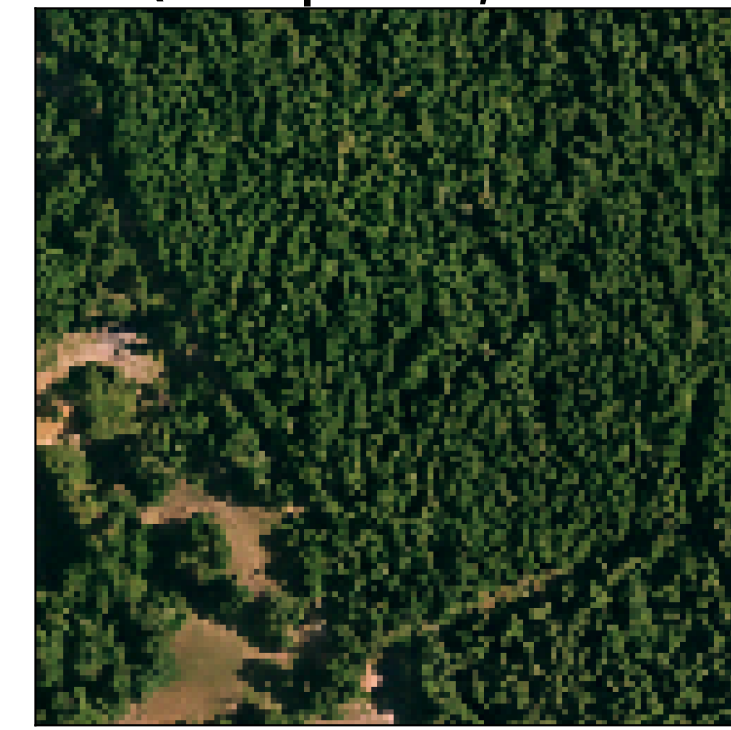
FM (Midpoint; n = 20 )
