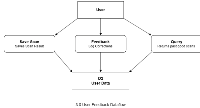
Figure 5: User Data and Feedback Flow
