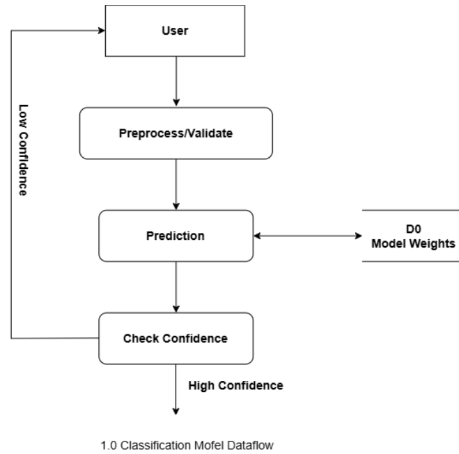
Figure 4: ML Classification Process
