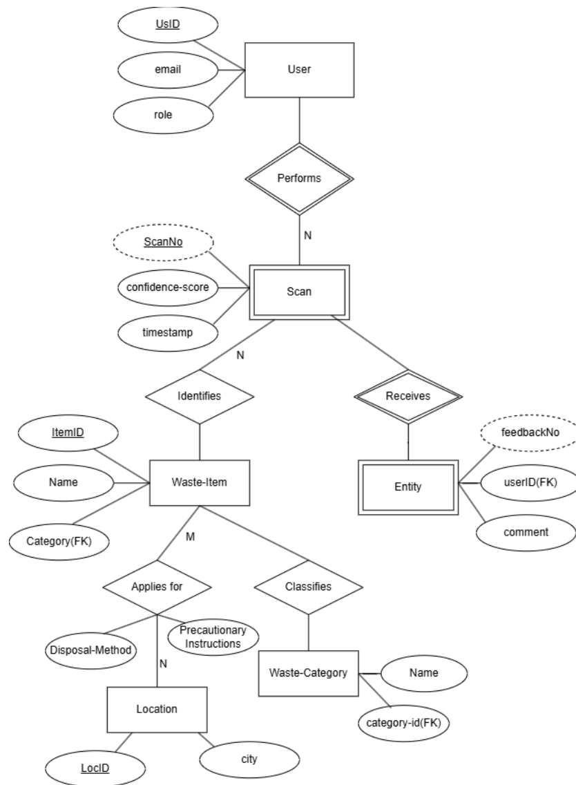
Figure 2.4: Entity Relationship Diagram for Sortify
