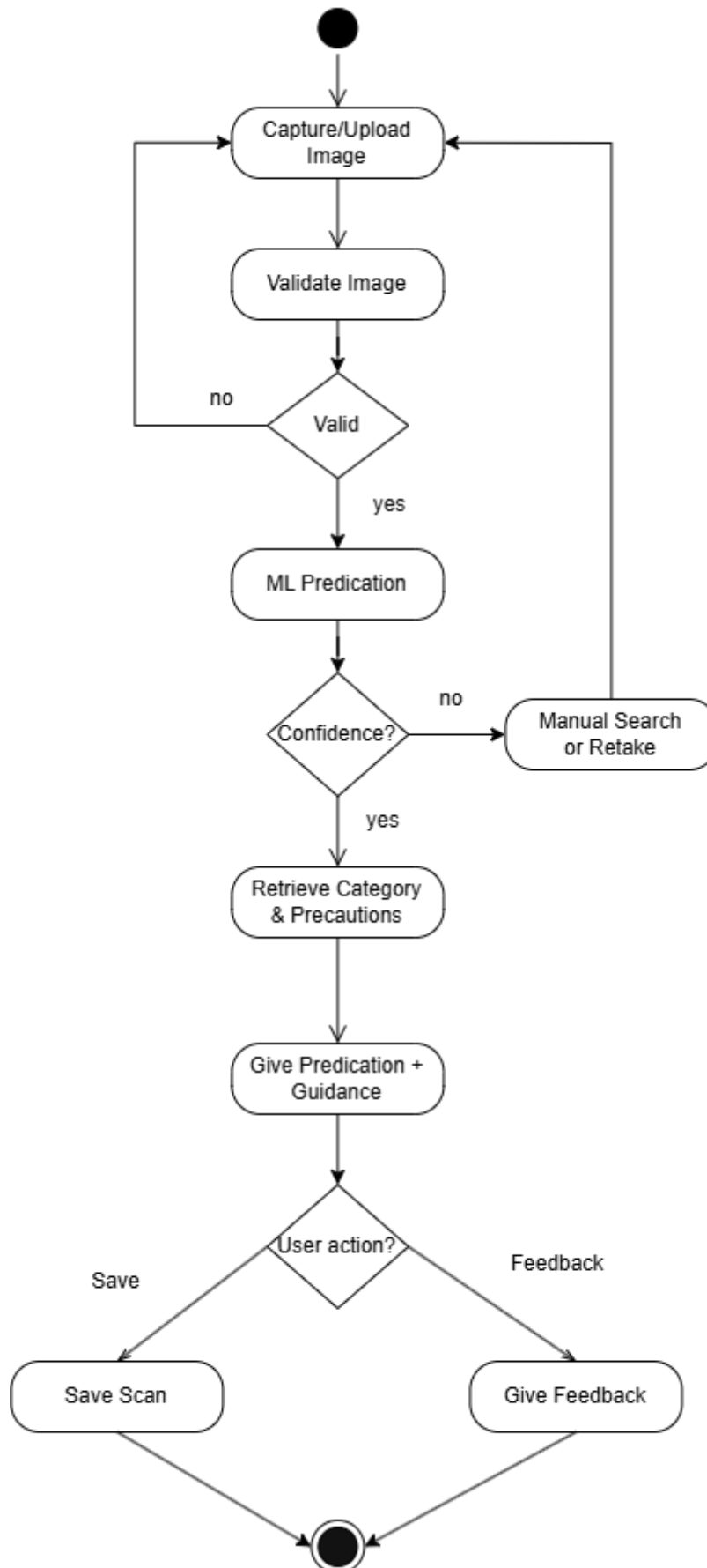
Figure 2.2: Activity Diagram for the Sortify Workflow
