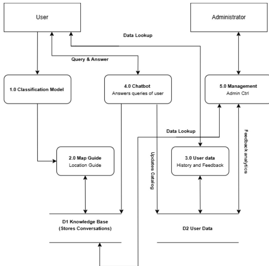
Figure 2.1: Level-1 Data Flow Diagram for Sortify
