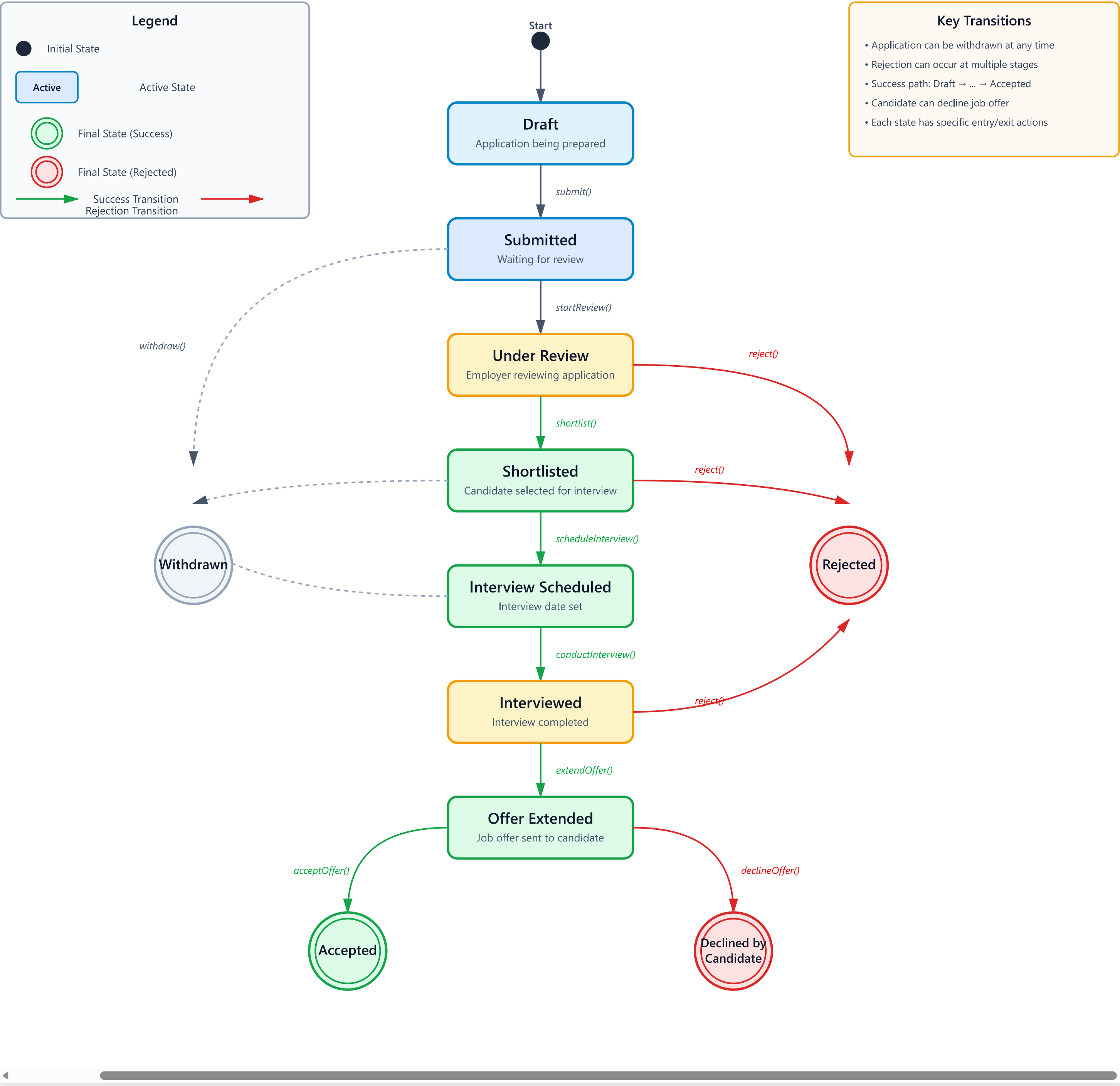
State Diagram - Job Application Lifecycle
