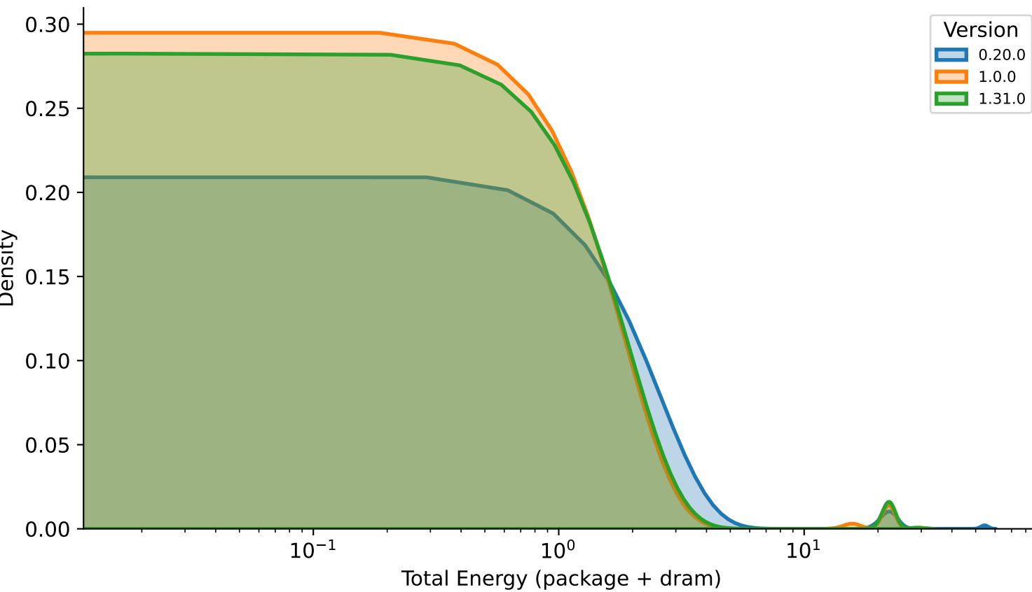
Polars — Adult Dataset
