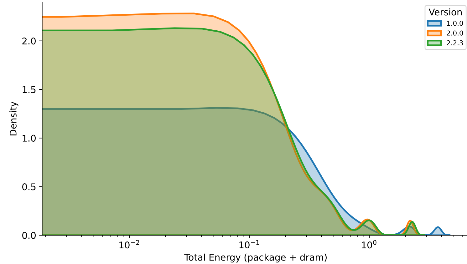
Vaex — Adult Dataset
