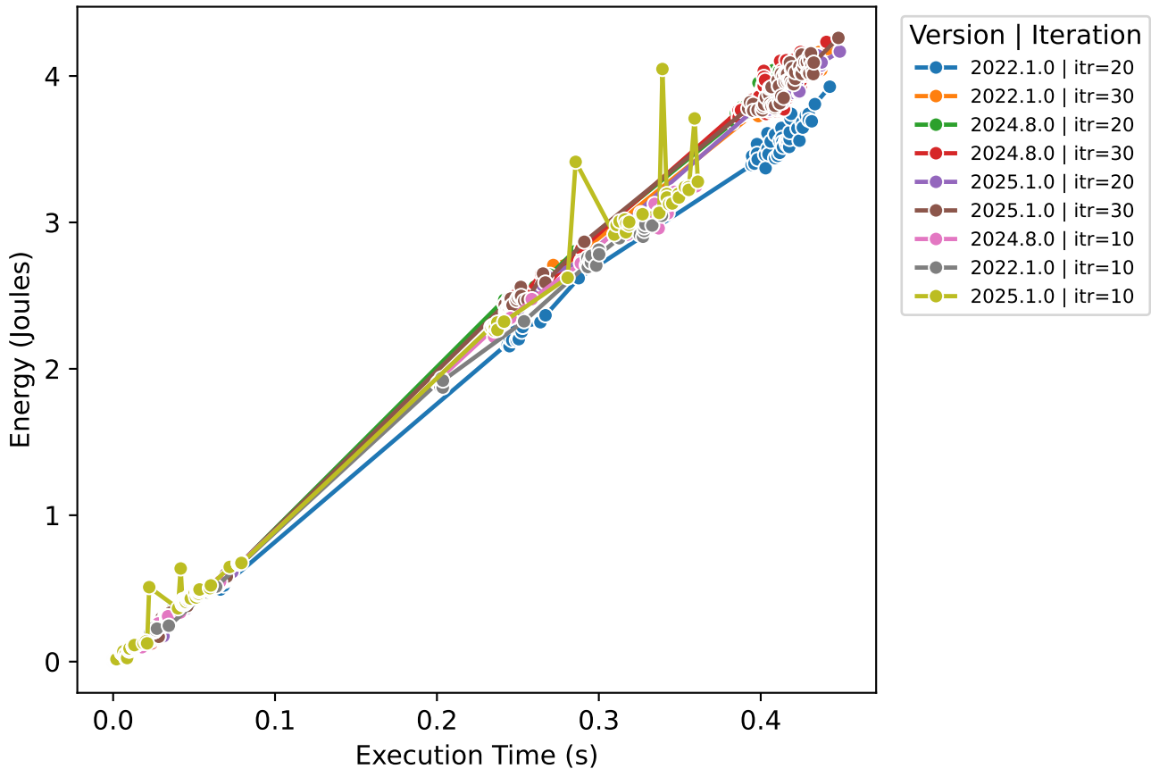
Execution Time vs Energy (Dask - Adult)
