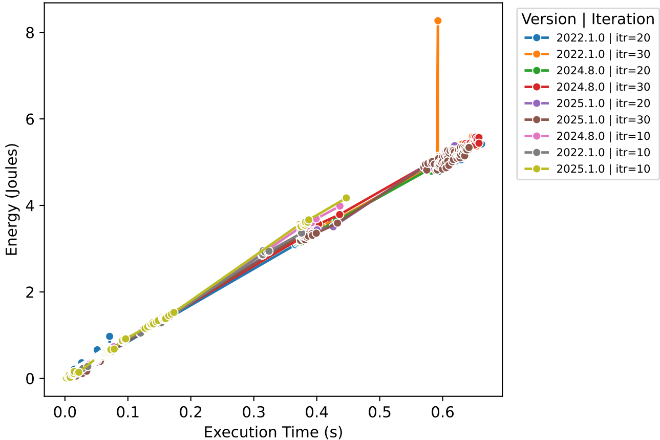
Execution Time vs Energy (Dask - Bank Marketing)
