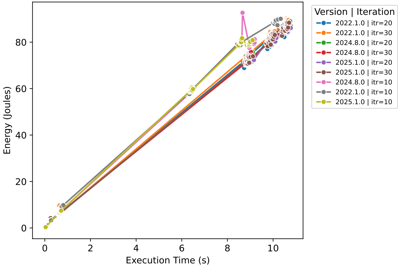
Execution Time vs Energy (Dask - Drug Review)
