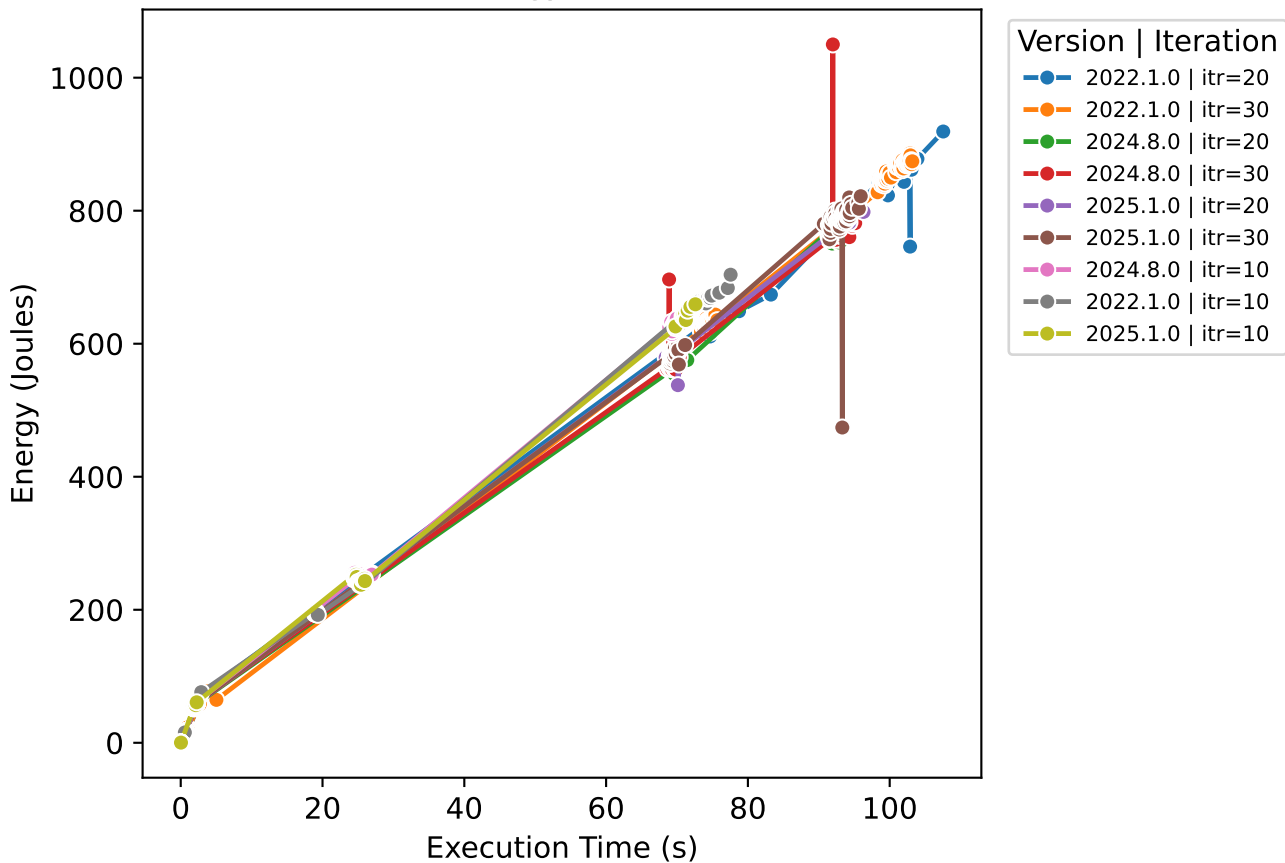
Execution Time vs Energy (Dask - US Census 1990)
