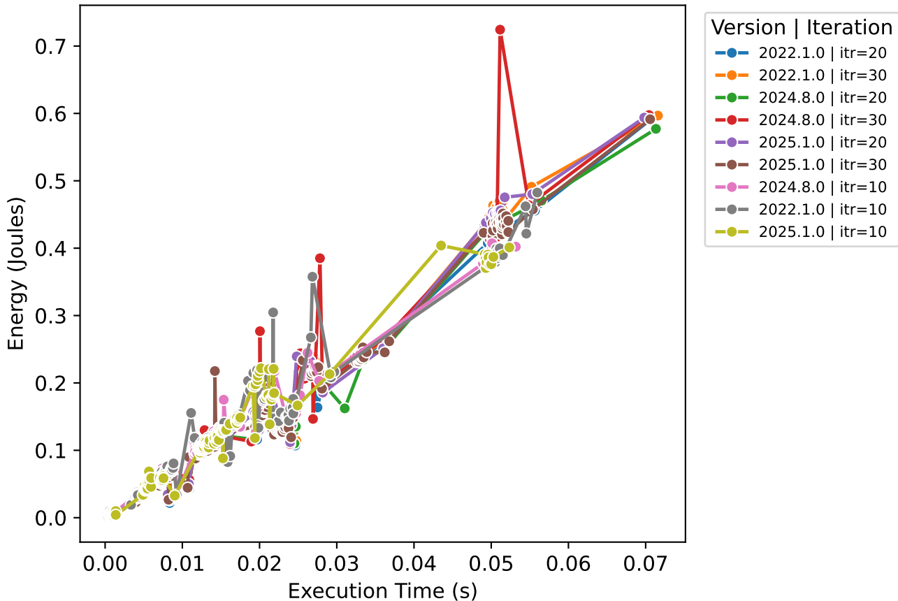
Execution Time vs Energy (Dask - Water Potability)
