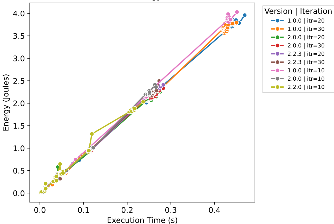
Execution Time vs Energy (Pandas - Adult)
