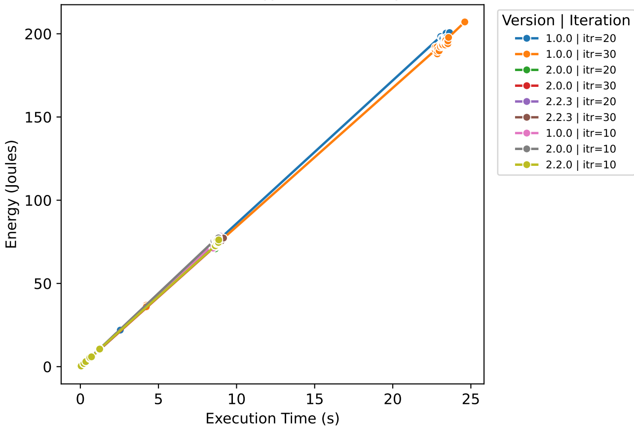
Execution Time vs Energy (Pandas - Drug Review)
