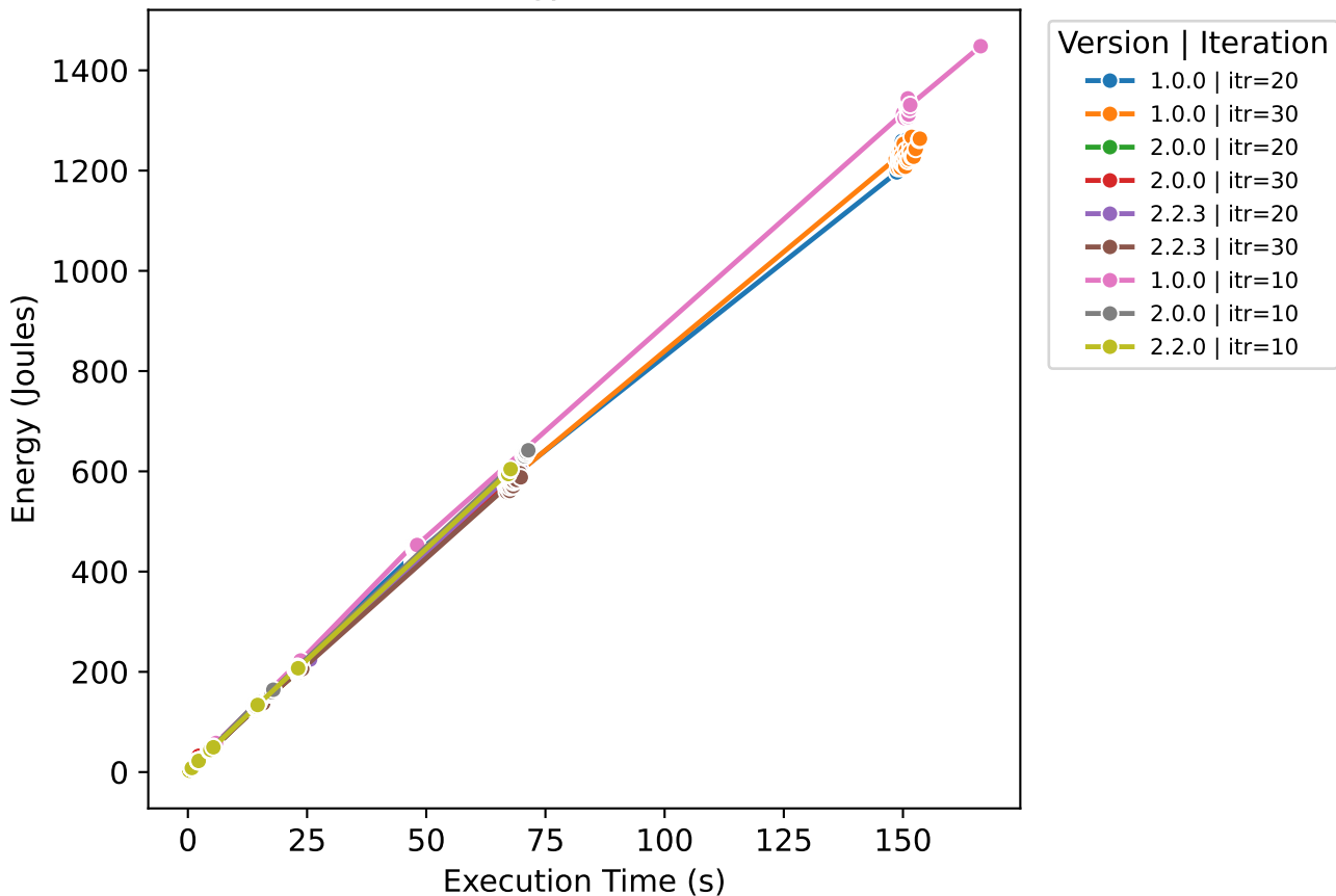
Execution Time vs Energy (Pandas - US Census 1990)
