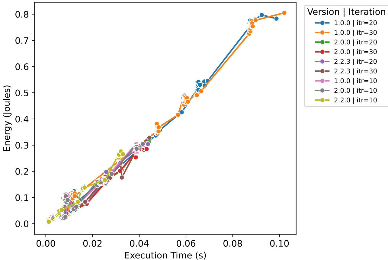
Execution Time vs Energy (Pandas - Water Potability)
