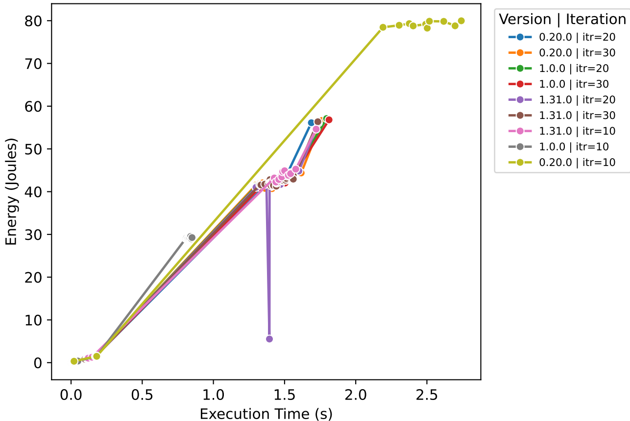
Execution Time vs Energy (Polars - Bank Marketing)
