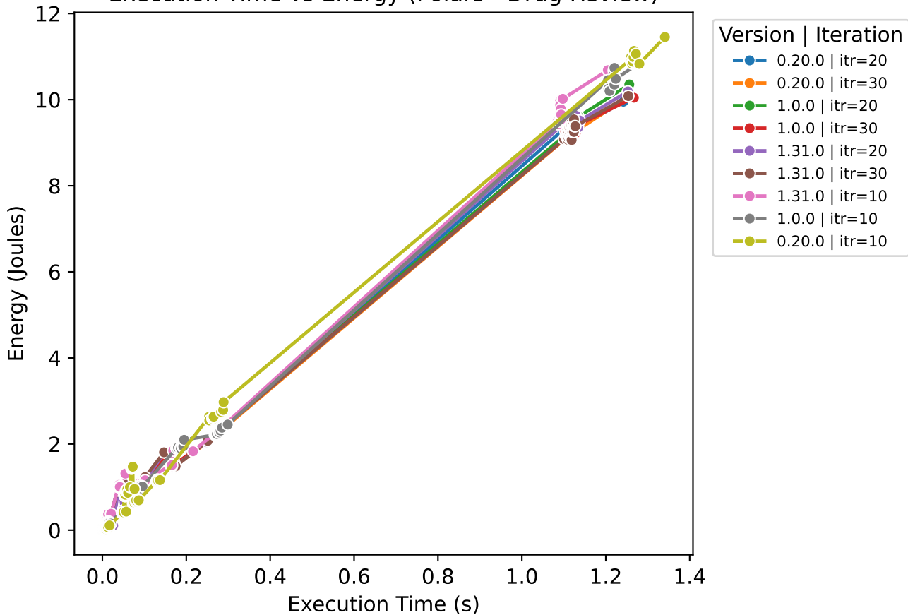
Execution Time vs Energy (Polars - Drug Review)
