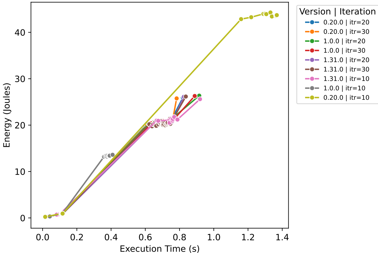
Execution Time vs Energy (Polaris - Student Exam)
