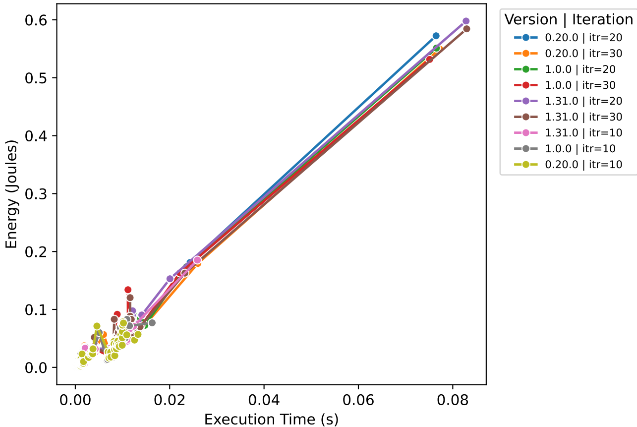
Execution Time vs Energy (Polars - Water Potability)
