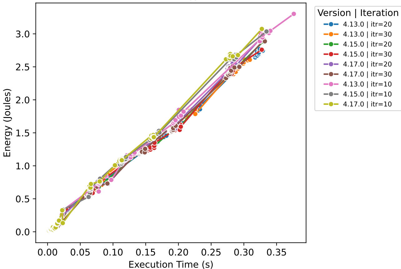
Execution Time vs Energy (Vaex - Adult)
