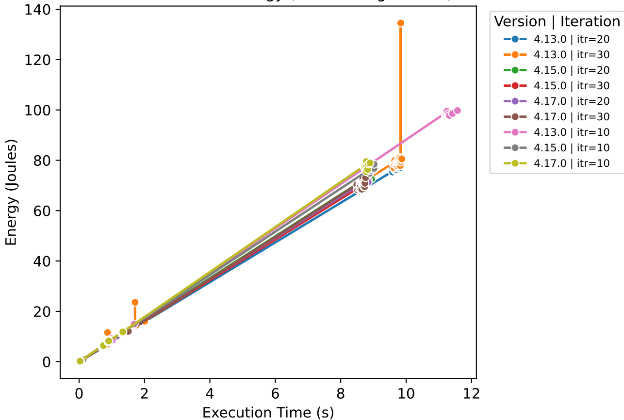
Execution Time vs Energy (Vaex - Drug Review)
