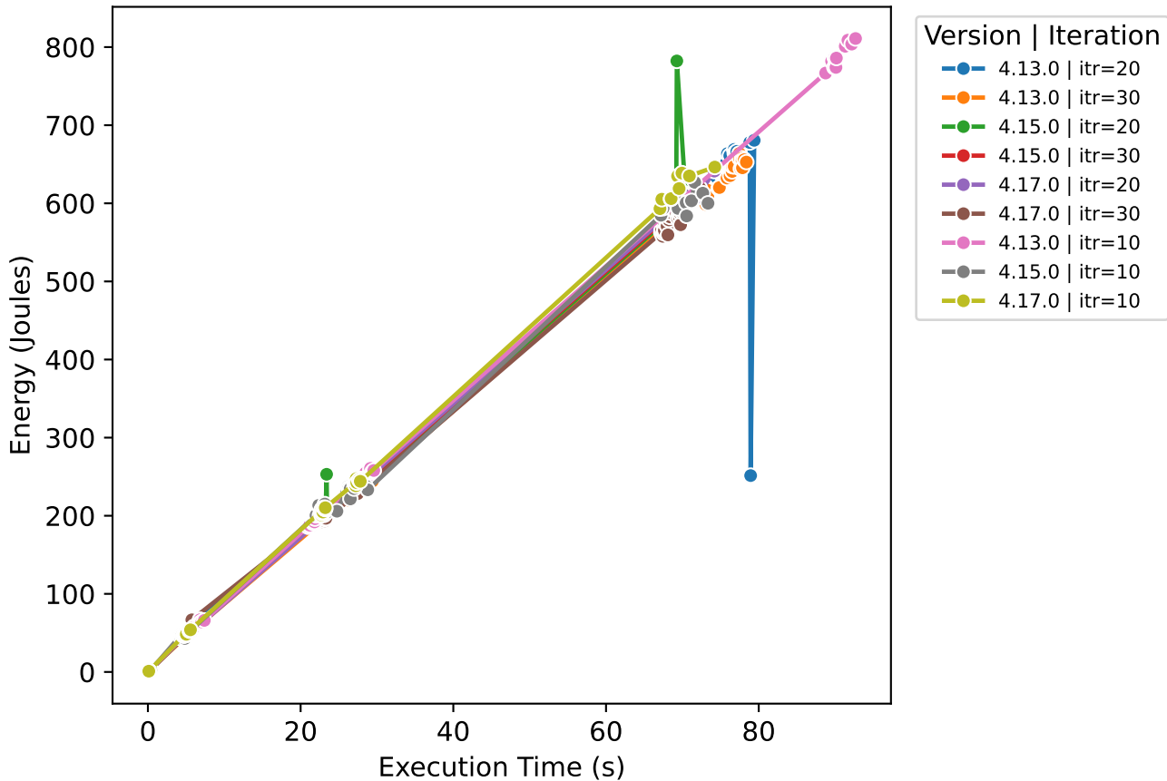
Execution Time vs Energy (Vaex - US Census 1990)
