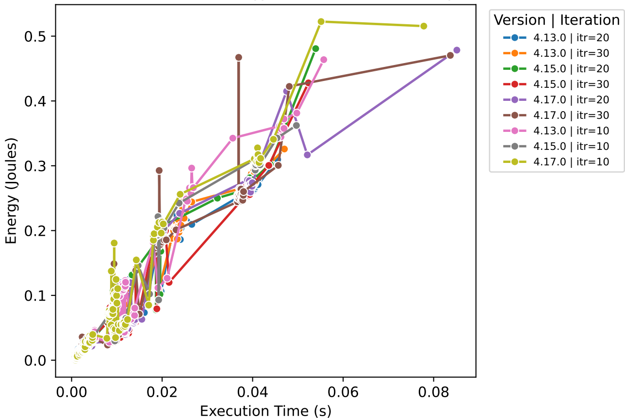
Execution Time vs Energy (Vaex - Water Potability)
