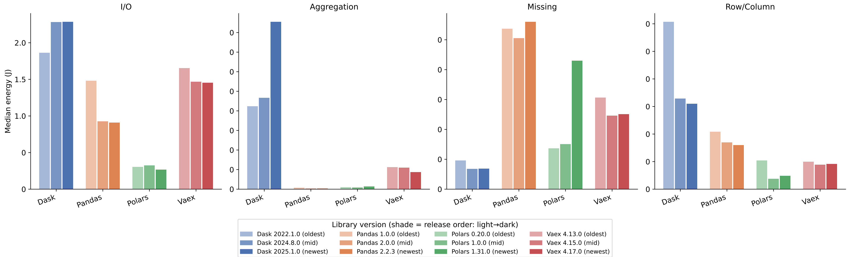
Median Energy Consumption by Library, Version & Operation Category (itr=10)
